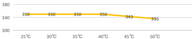
Temperature (Celsius) Derate Curves Unit: kVA
